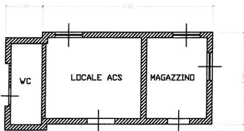
PIANO TERRA h 2.80
